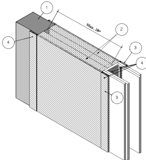
Installation in Gypsum/Steel Stud Wall or Concrete Wall Construction
