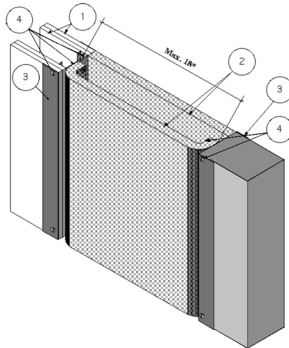
Installation in Gypsum/Steel Stud Wall or Concrete Wall Construction
