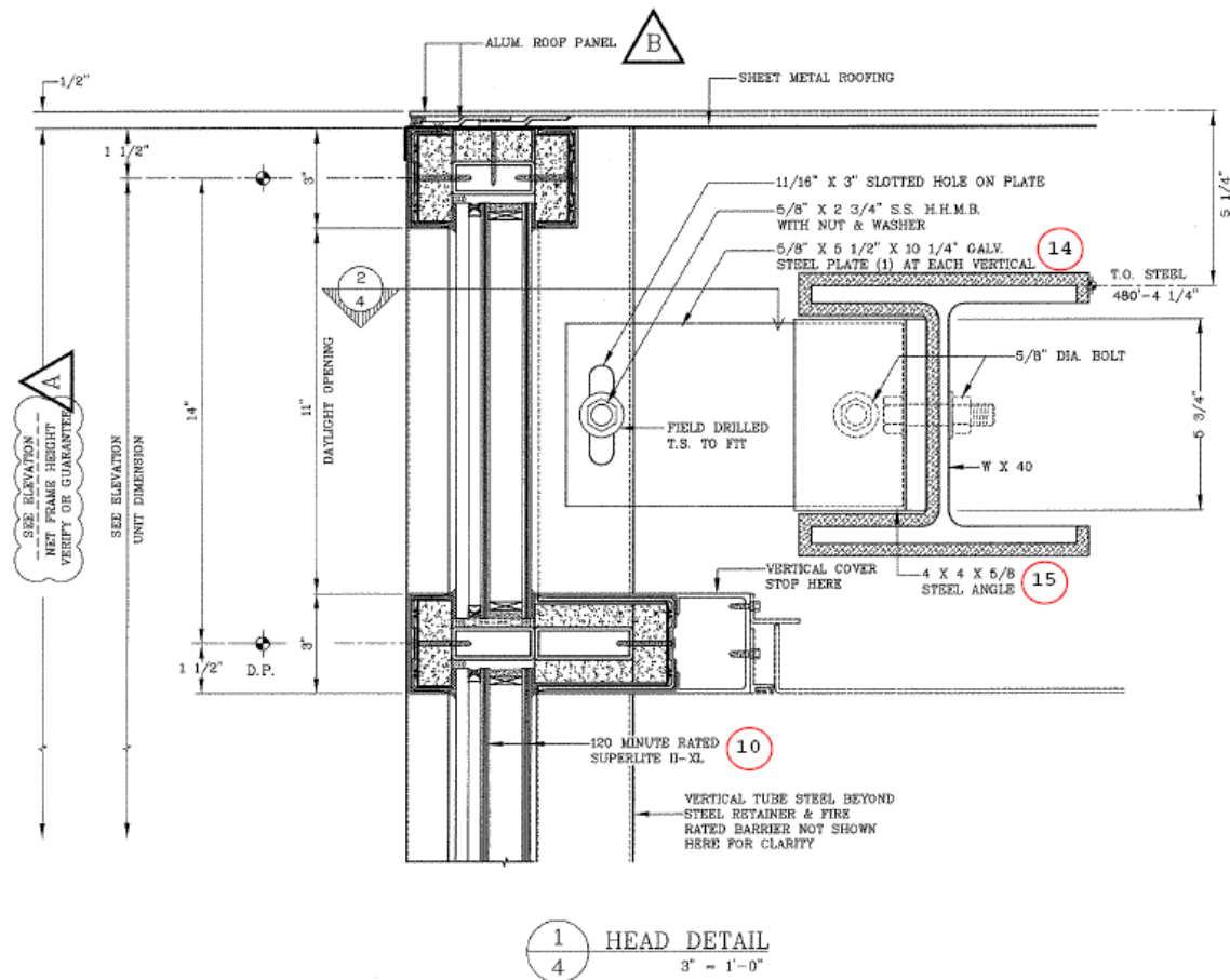
Figure 3. Head Details.
