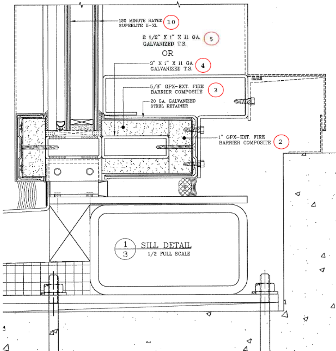
Figure 6. Sill Detail.
