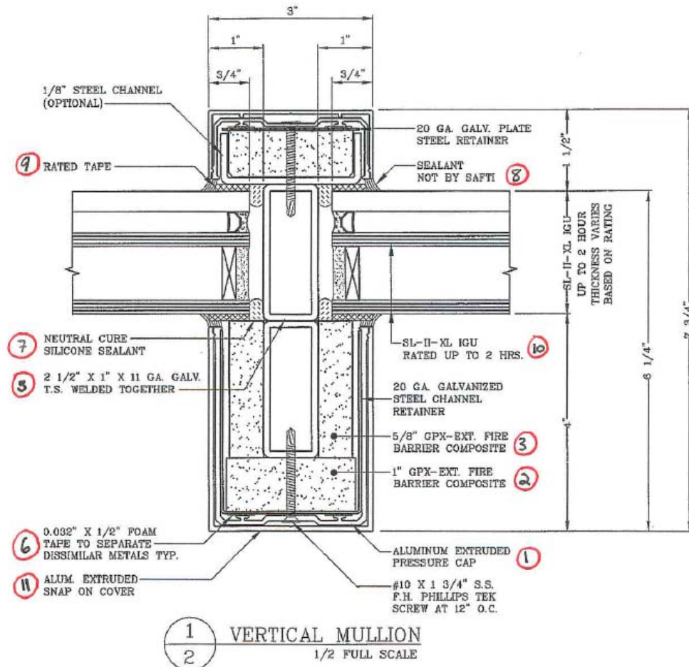
Figure 1A. Alternate Vertical Mullion Details.
