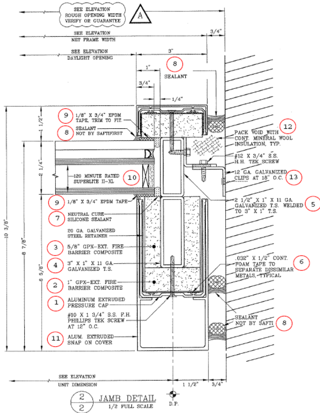
Figure 2. Jamb Details.
