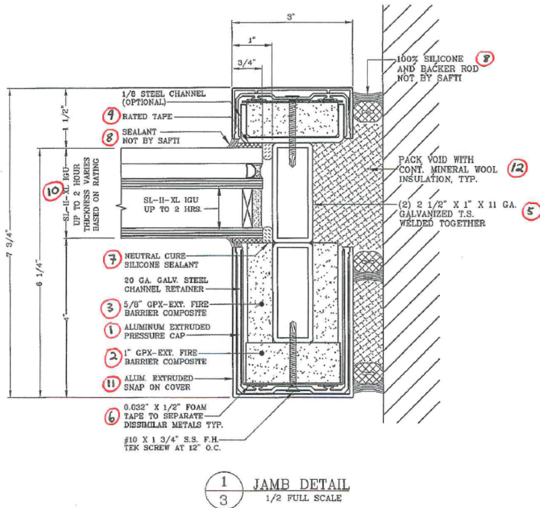
Figure 2A. Alternate Jamb Details.
