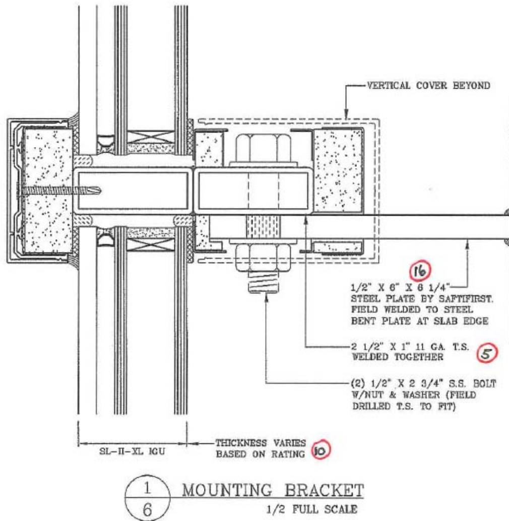
Figure 4A. Alternate Mounting Bracket Details.
