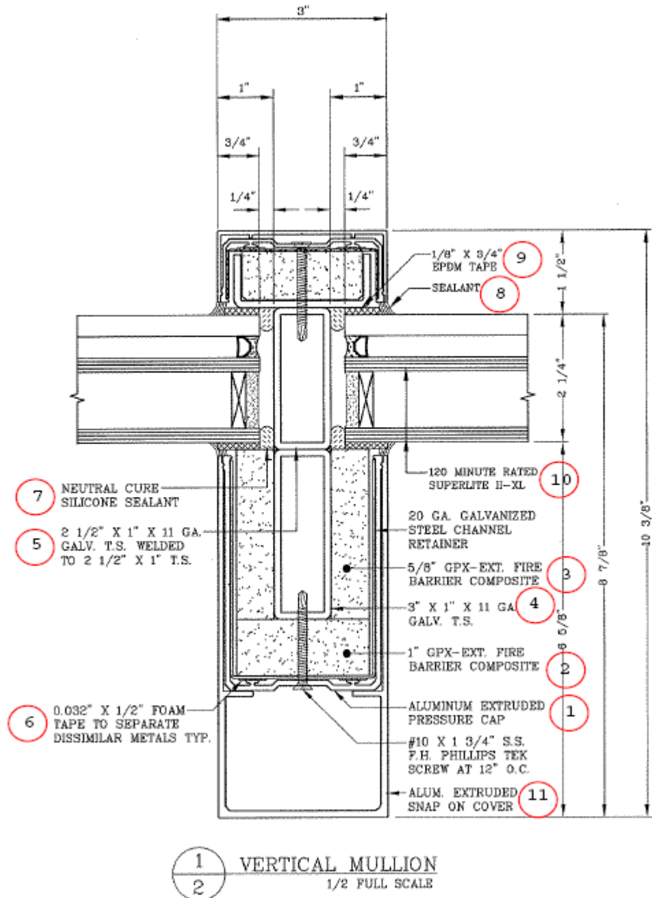
Figure 1. Vertical Mullion Details.
