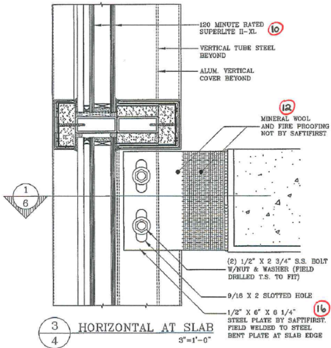
Figure 5. Horizontal at Slab Details.
