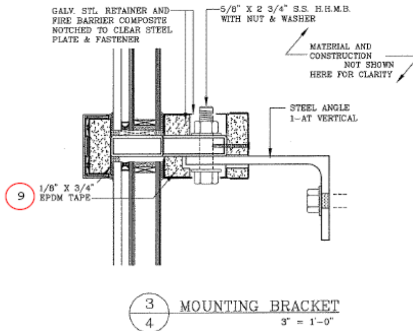
Figure 4. Mounting Bracket Details.
