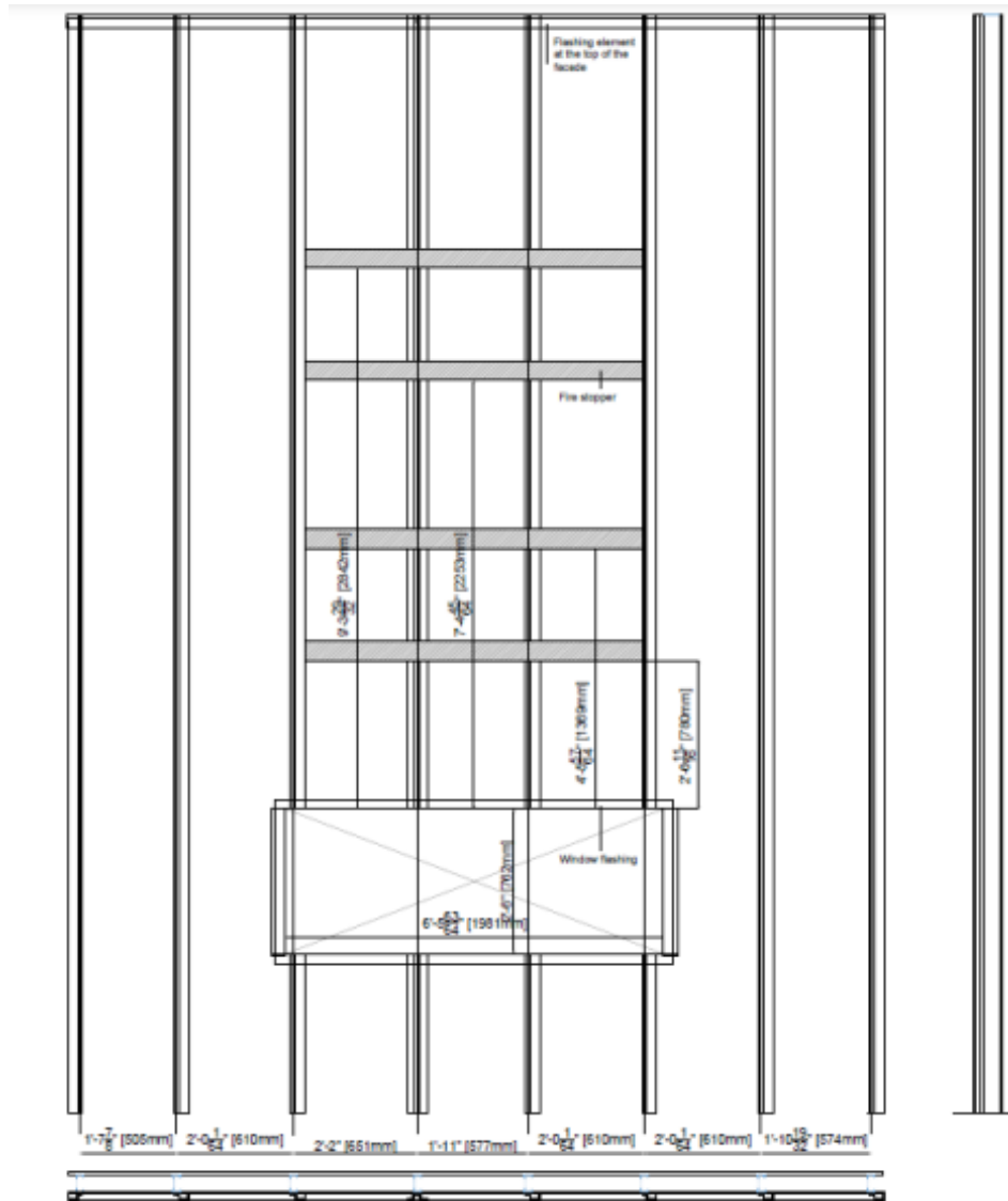
Figure 2 – Placement of Fire Barrier
