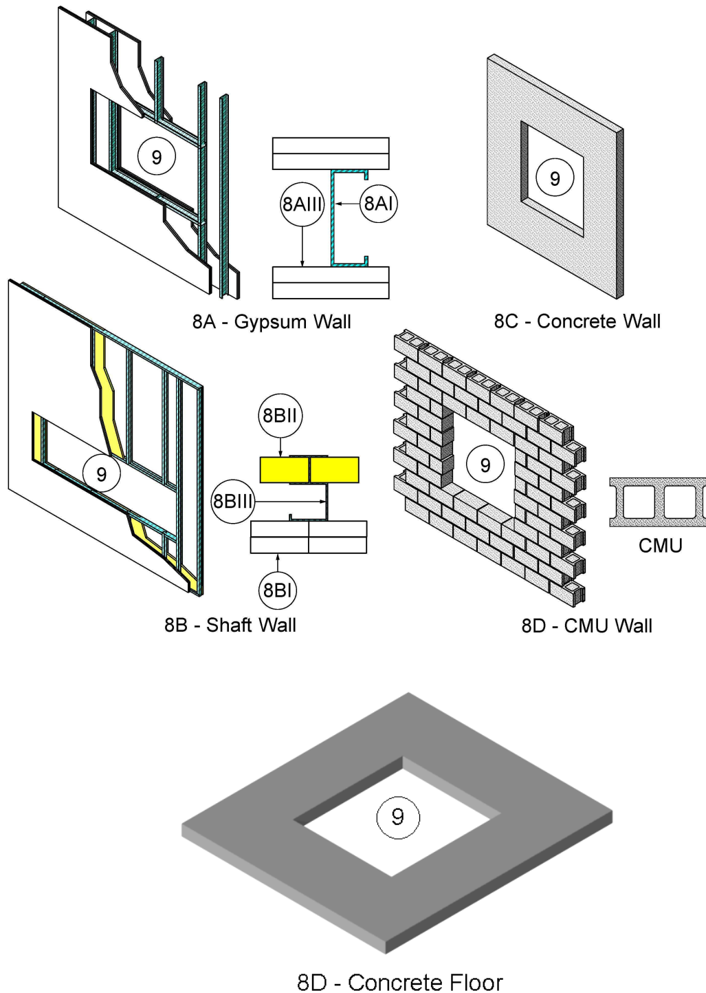
Figure 5 – Noncombustible Supporting Constructions
