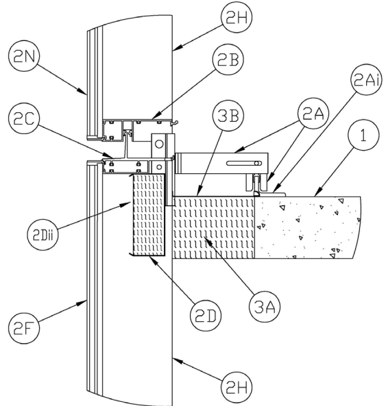
Figure 3 - Base Detail at Anchor
