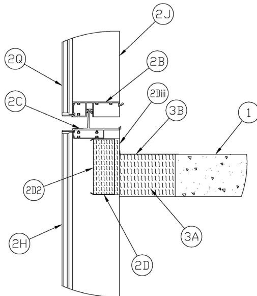
Figure 8 - Base Detail Interior Backpan Insulation
