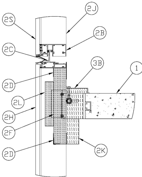
Figure 4 - Base Detail at Anchor (Jamb)
