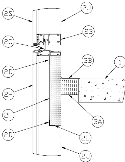
Figure 2 - Base Detail Between Anchors
