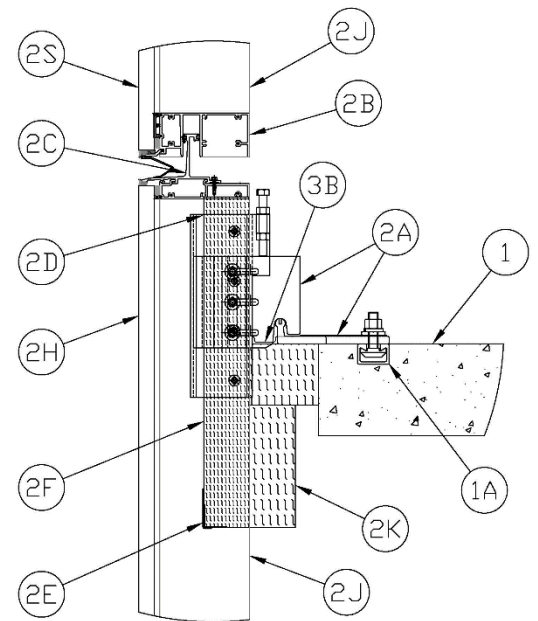
Figure 5 - Base Detail at Anchor (Top of Slab)
