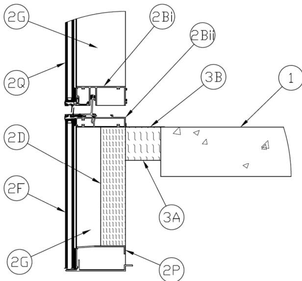
Figure 8 - Windload Anchor Configuration
