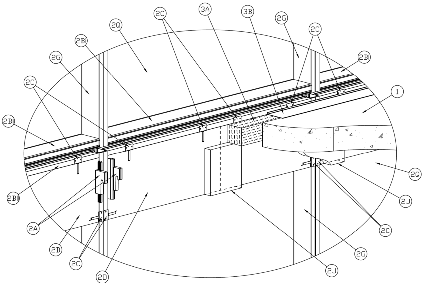
Figure 1 - Isometric with Interior Vertical Mullion Detail
