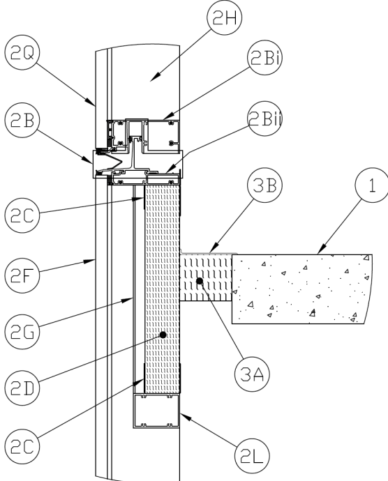
Figure 6 - Kiss Transom Configuration
