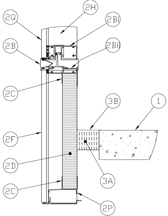
Figure 9 - Windload Anchor Configuration
