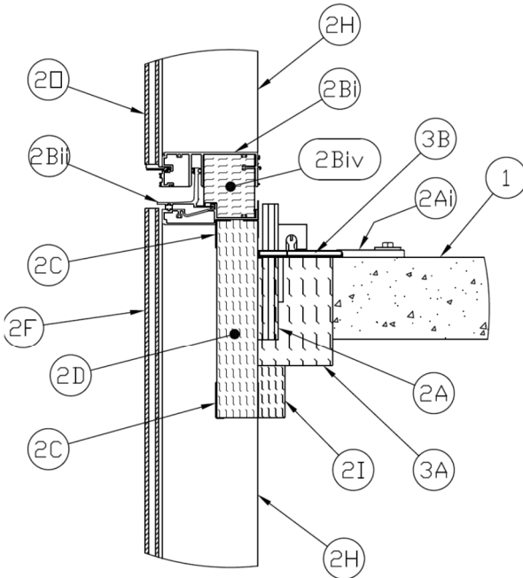
Figure 2 - Base Detail Between Anchors
