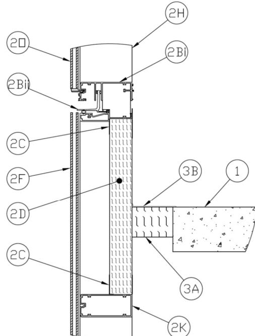
Figure 3 - Base Detail at Anchor (Face Mounted)
