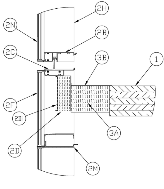
Figure 7 -Windload Anchor Configuration
