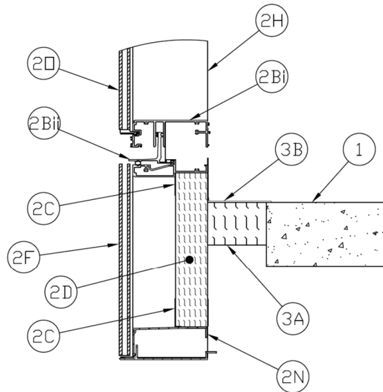
Figure 7 - Intermediate Transom with Shadowbox Configuration
