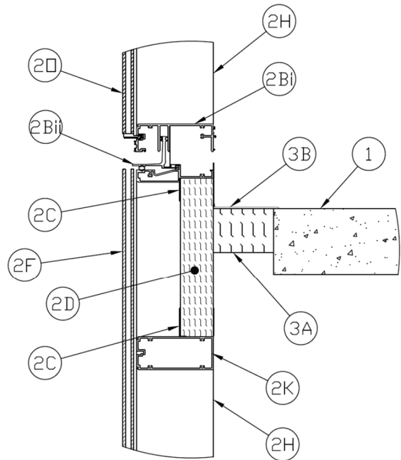
Figure 3 - Base Detail at Anchor (Face of Slab)
