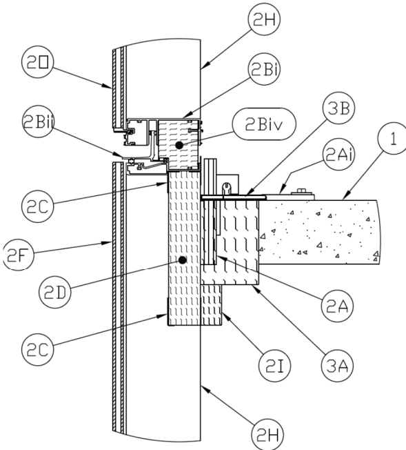
Figure 2 - Base Detail Between Anchors
