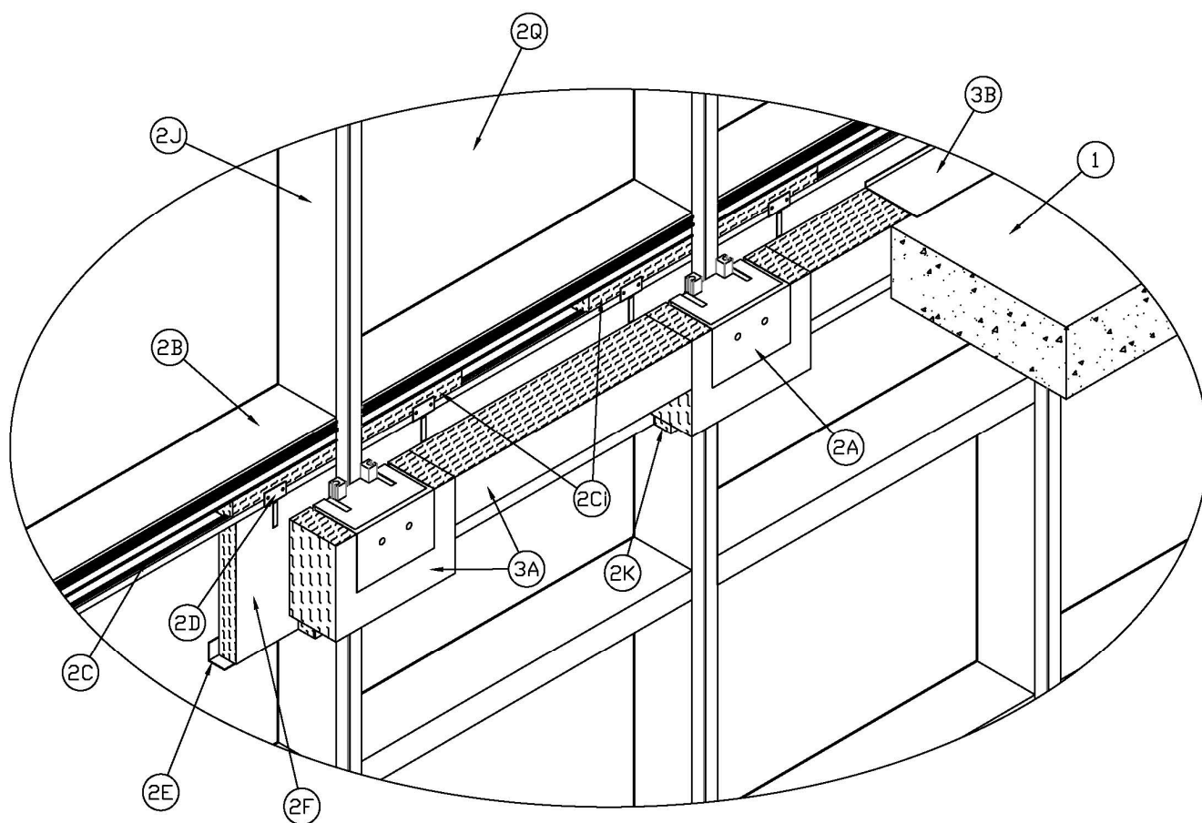
Figure 1 - Isometric with Interior Vertical Mullion Detail
