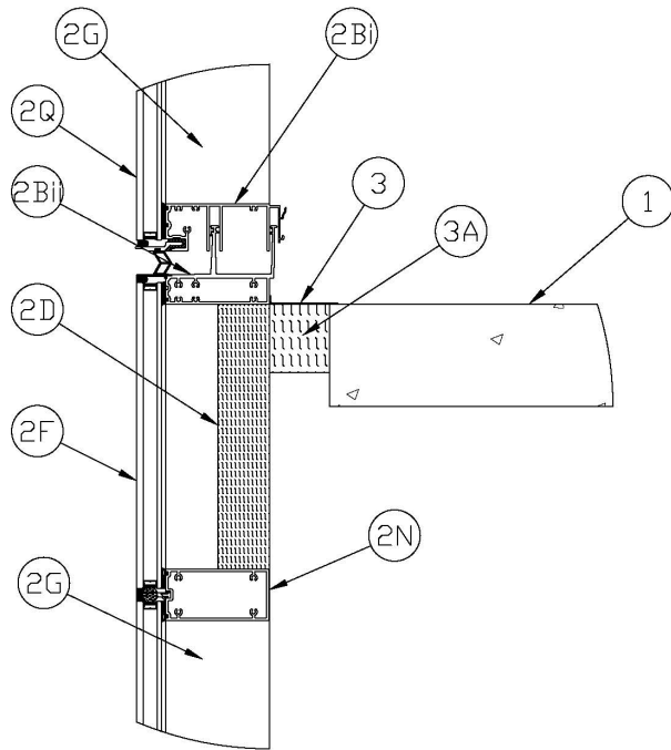
Figure 6 - Base Detail Between Anchors (Captured Transom)
