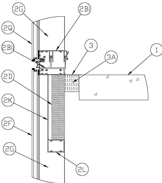
Figure 4 - Base Detail Intermediate Transom with Shadow Box
