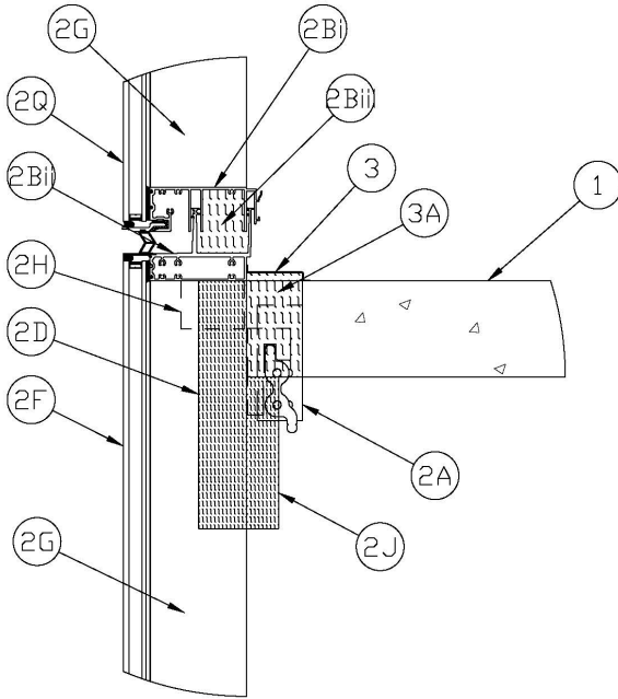
Figure 2 - Base Detail at Anchors
