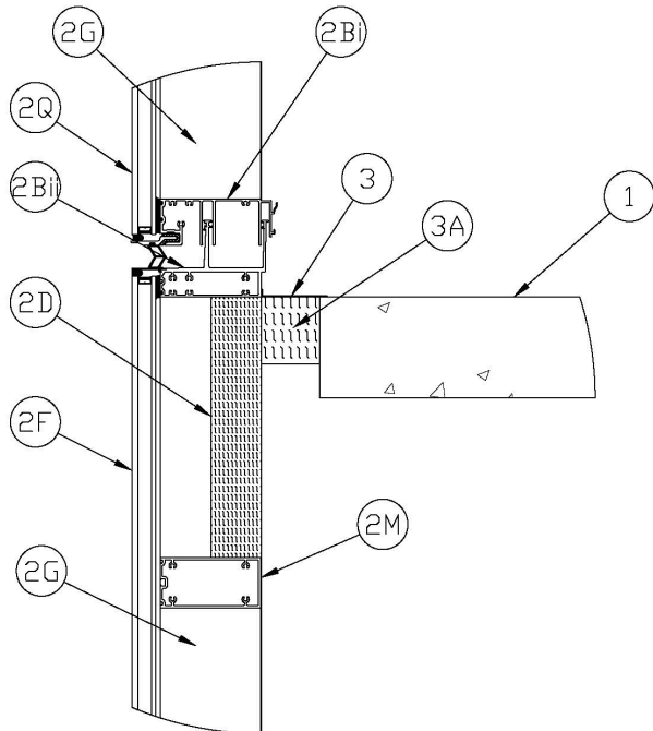
Figure 5 - Base Detail Between Anchors (Kiss Transom)
