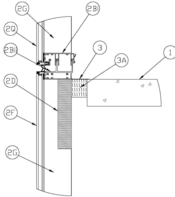
Figure 3 - Base Detail Between Anchors
