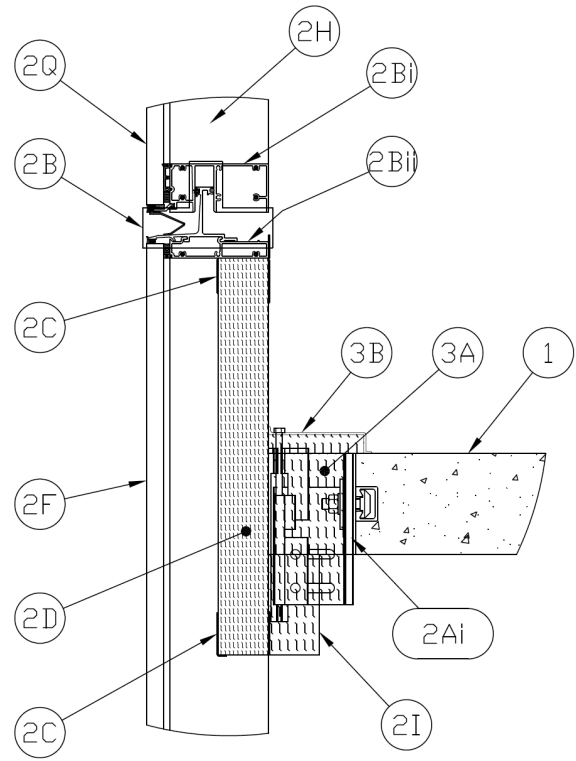
Figure 3 - Base Detail at Anchor (Face of Slab)
