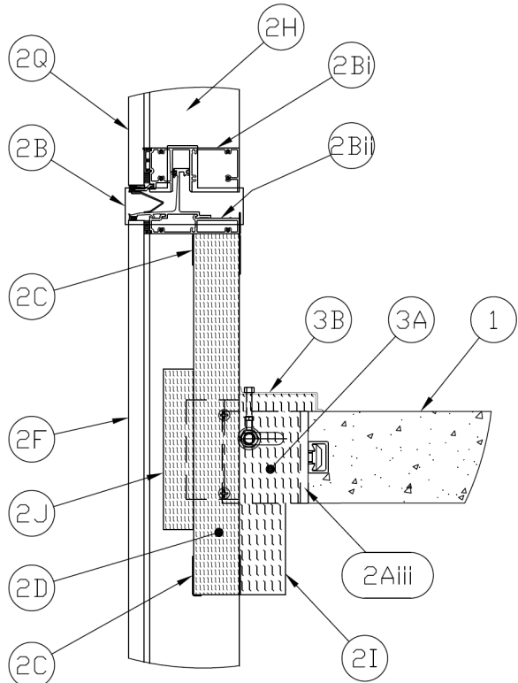
Figure 3 - Base Detail at Anchor (Face of Slab)
