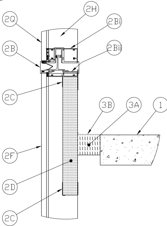
Figure 2 - Base Detail Between Anchors
