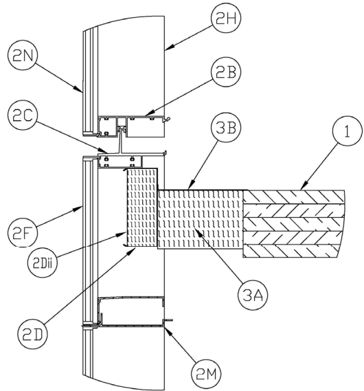
Figure 7 - Windload Anchor Configuration
