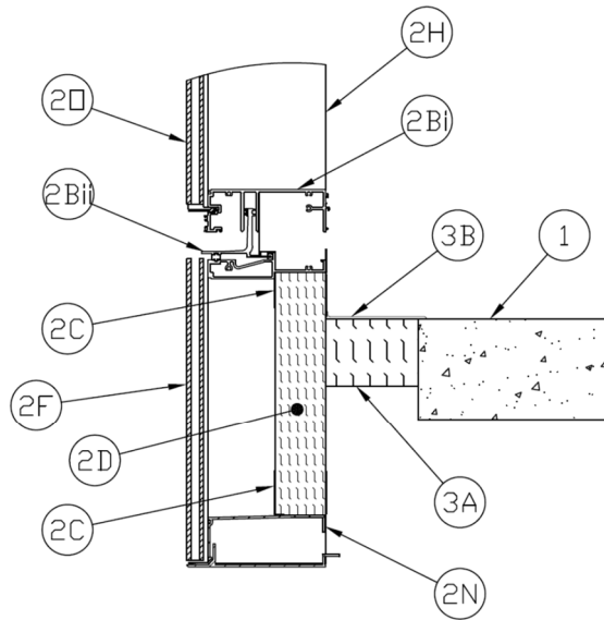
Figure 6 - Captured Transom Configuration
