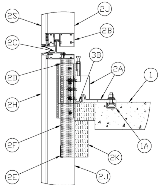
Figure 5 - Base Detail at Anchor (Top of Slab)
