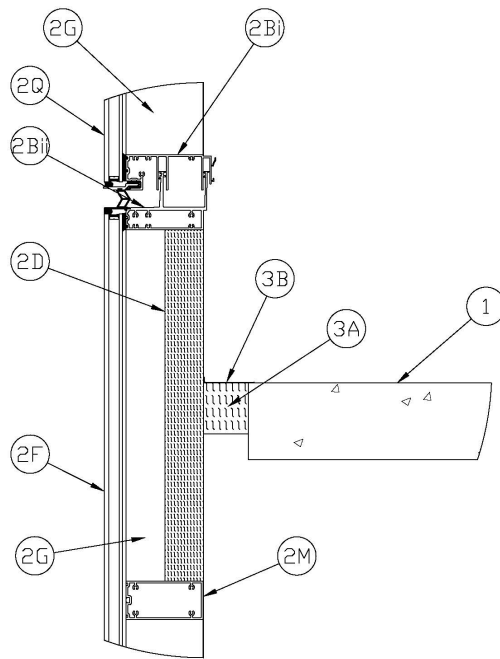
Figure 5 - Base Detail Between Anchors (Kiss Transom)
