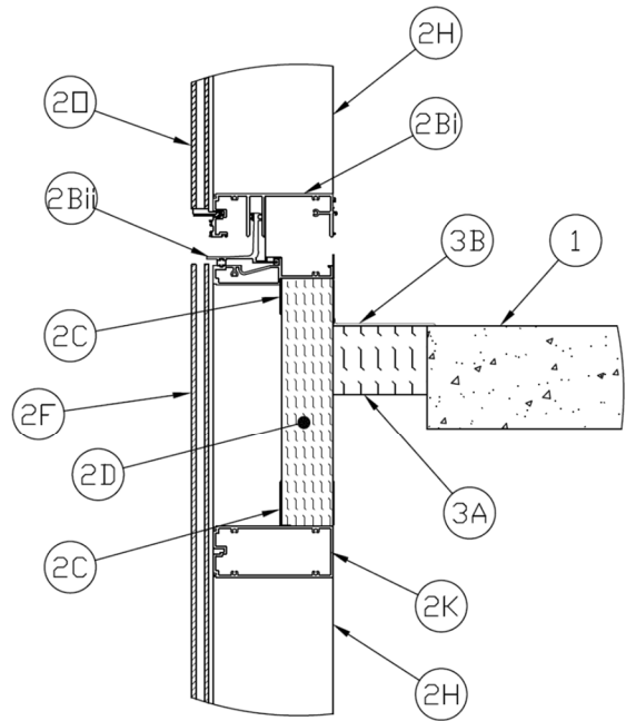
Figure 3 - Base Detail at Anchor (Face of Slab)
