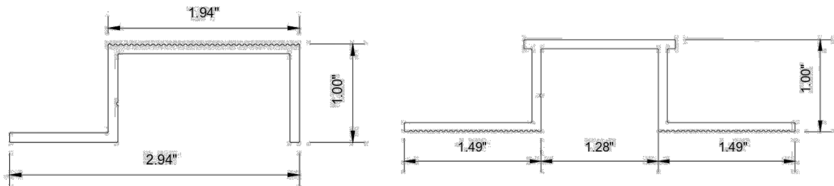
Figure 3 – J- and H-Section Studs
