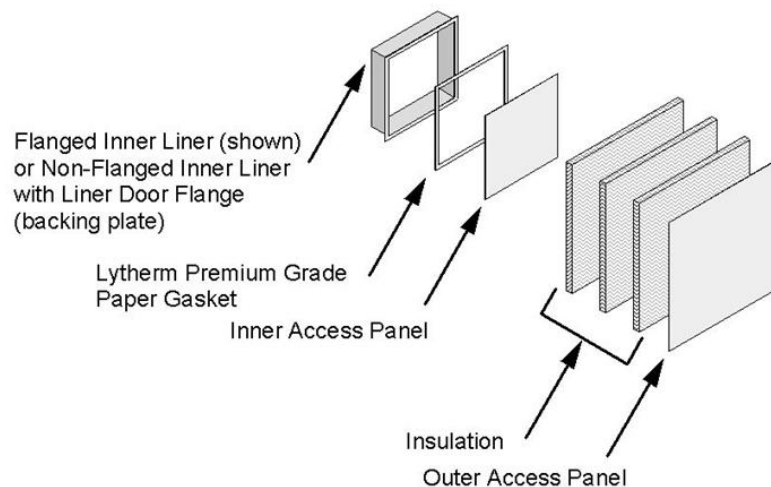
Figure 2. Access Door
