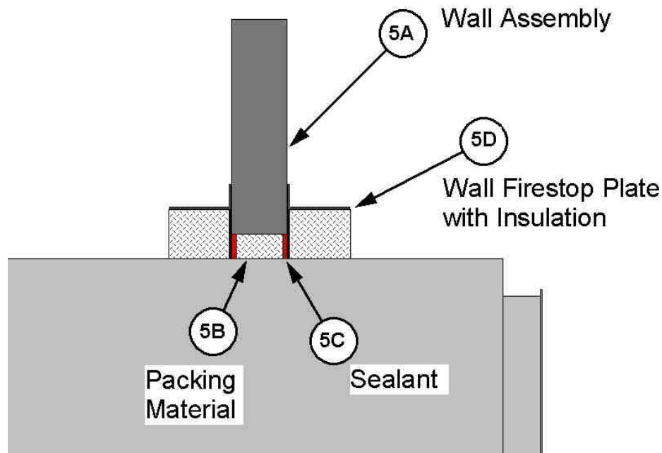
Figure 7. Wall Firestop
