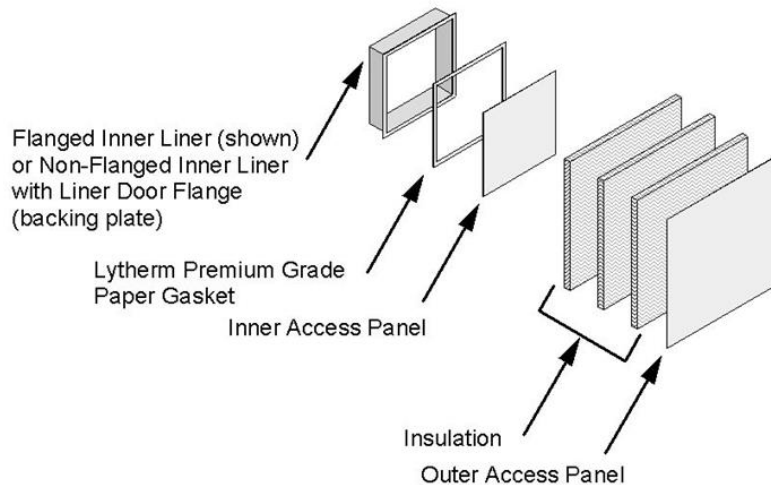
Figure 2. Access Door
