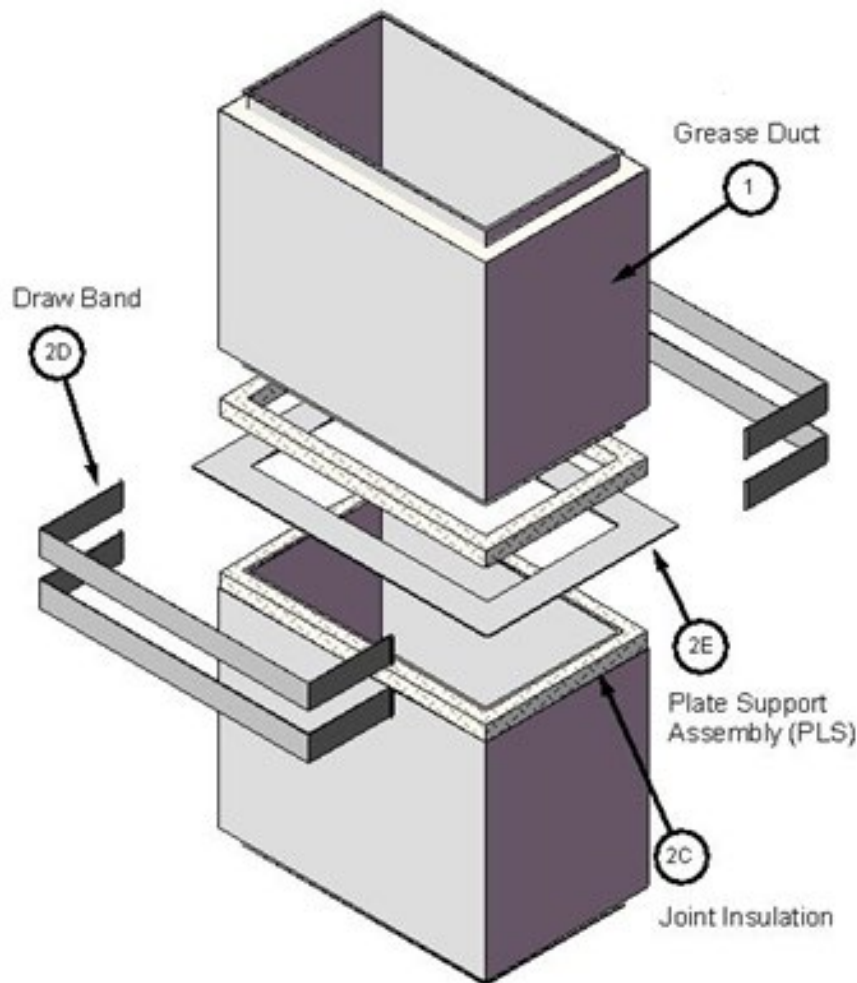
Figure 3. Plate Support Assembly (PLS)
