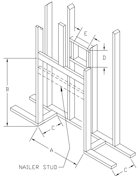
Figure 5: Framing
