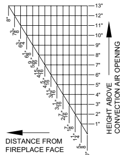
APPROVED MANTEL PROFILE
