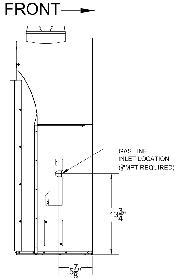
Figure 8: Gas Supply
