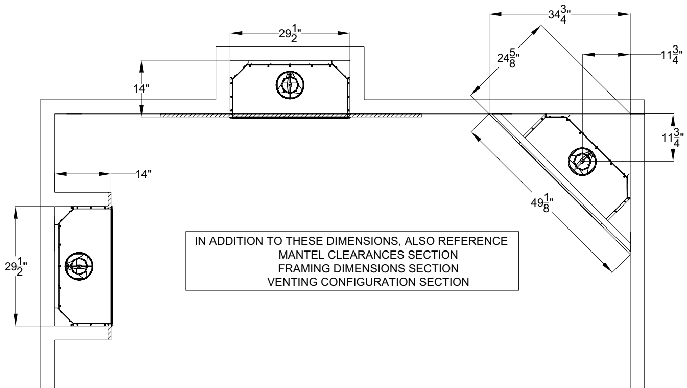
Figure 4: Planning Installation
