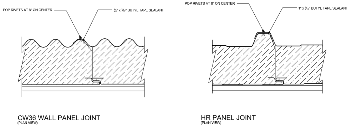
Figure 1 – Joint and Corrugation Profiles
