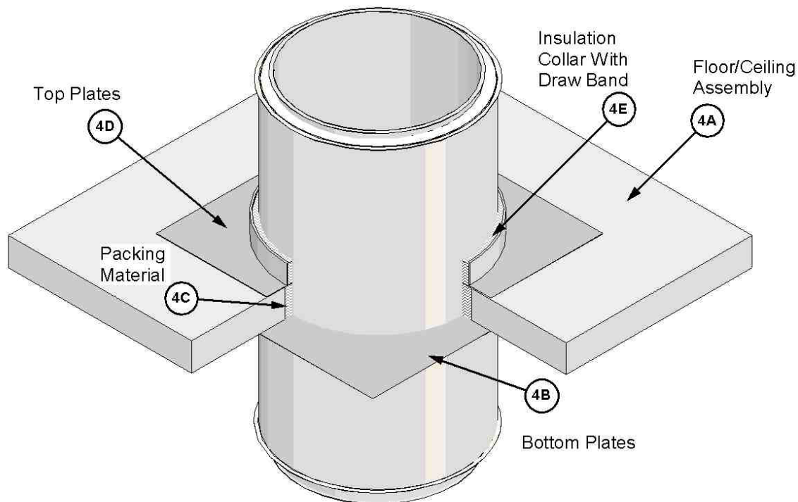
Figure 11: Floor/Ceiling Firestop
