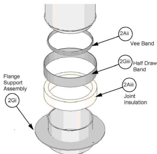
Figure 9. WFA Joint
