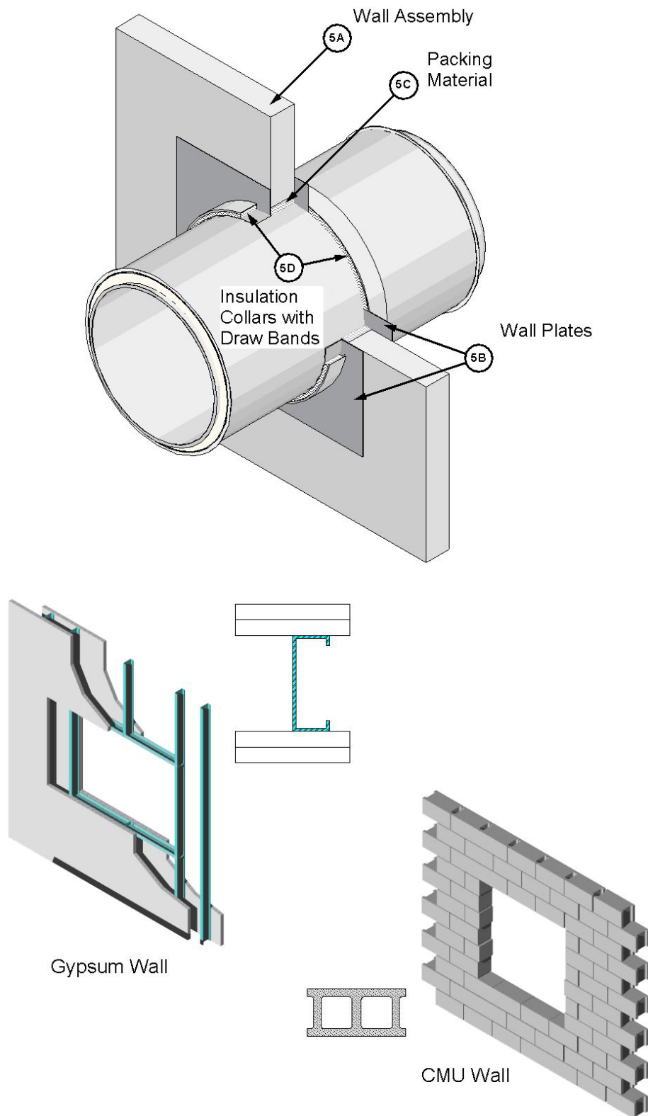
Figure 12. Wall Firestop
