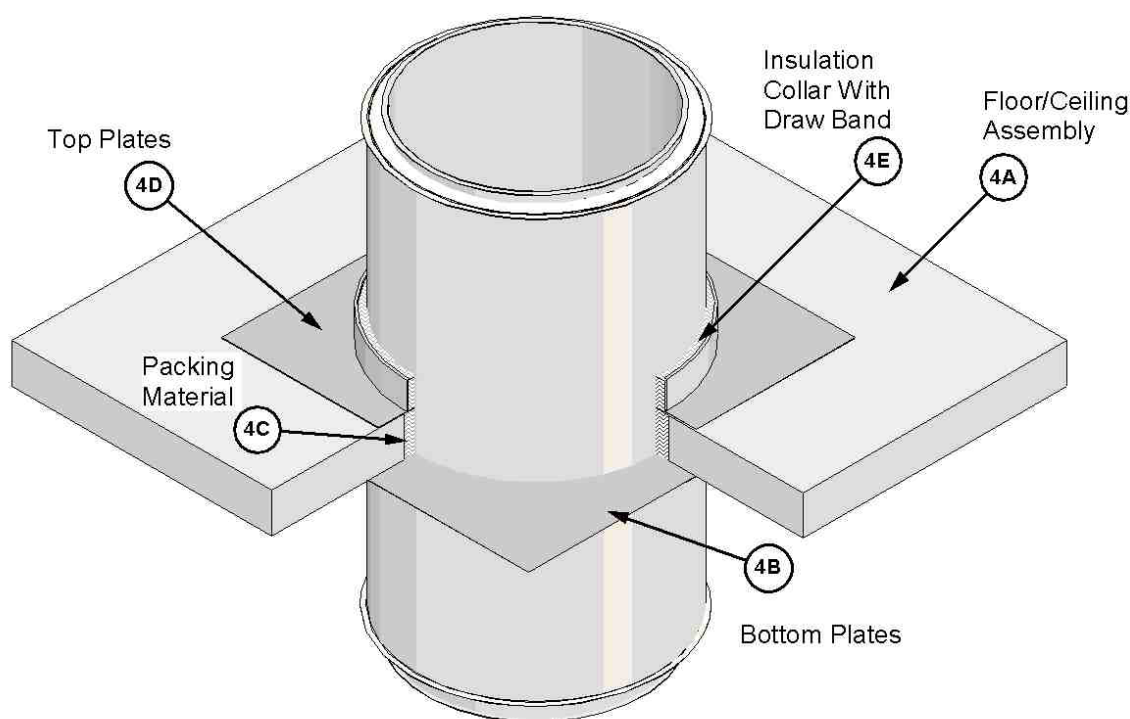
Figure 11: Floor/Ceiling Firestop
