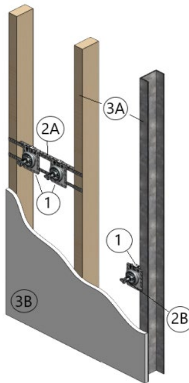
Figure 1. HR-FR Fixture Outlet Boxes in 1 Hour Fire Rated Walls
