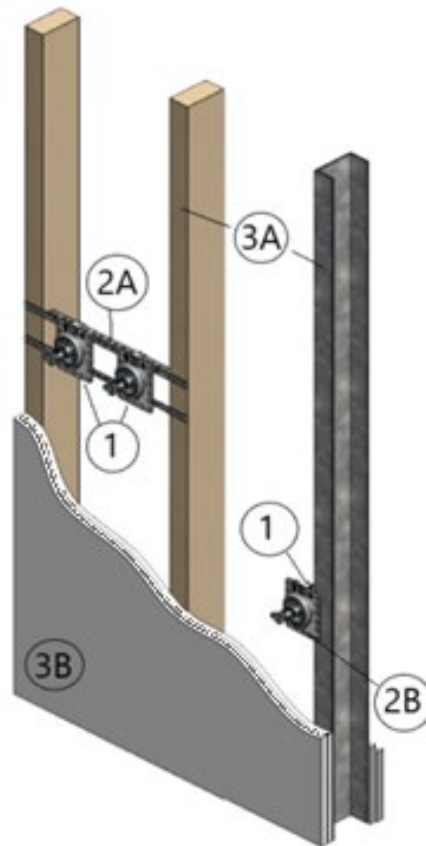
Figure 1. HR-FR Fixture Outlet Boxes in 2 Hour Fire Rated Walls
