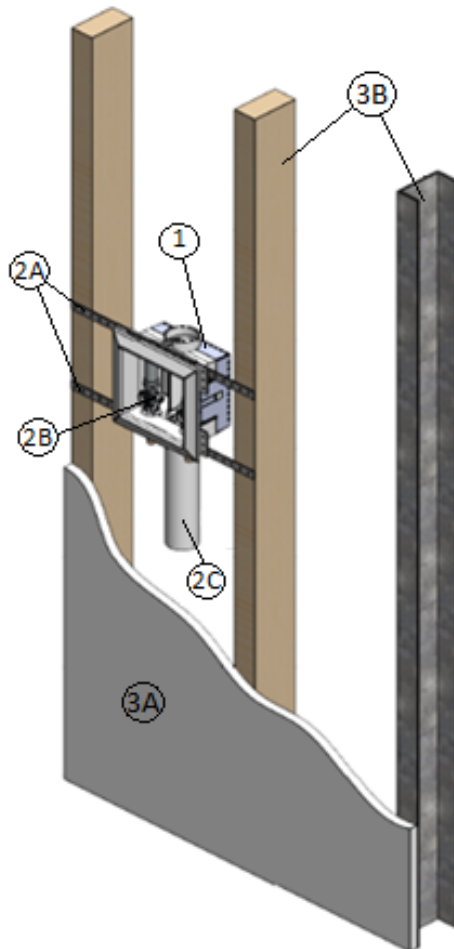
Figure 1. HR-WR Washing Machine Outlet Box in 1 Hour Fire Rated Walls
