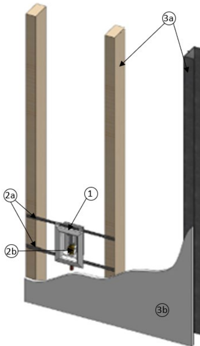
Figure 1. Outlet Box in 1 Hour Fire Rated Walls
