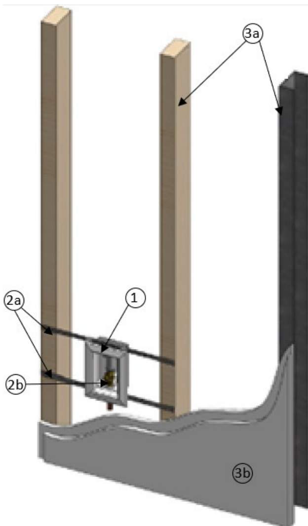
Figure 1. Outlet Box in 2 Hour Fire Rated Walls
