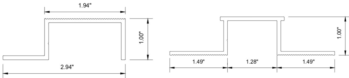
Figure 3 – J- and H-Section Studs
