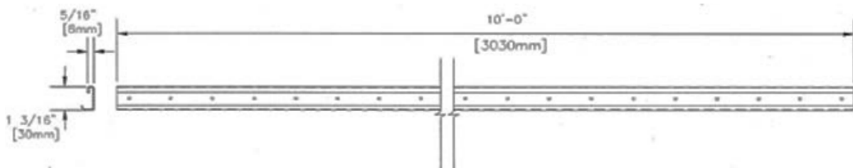
Figure 2 - Starter Track Profile
