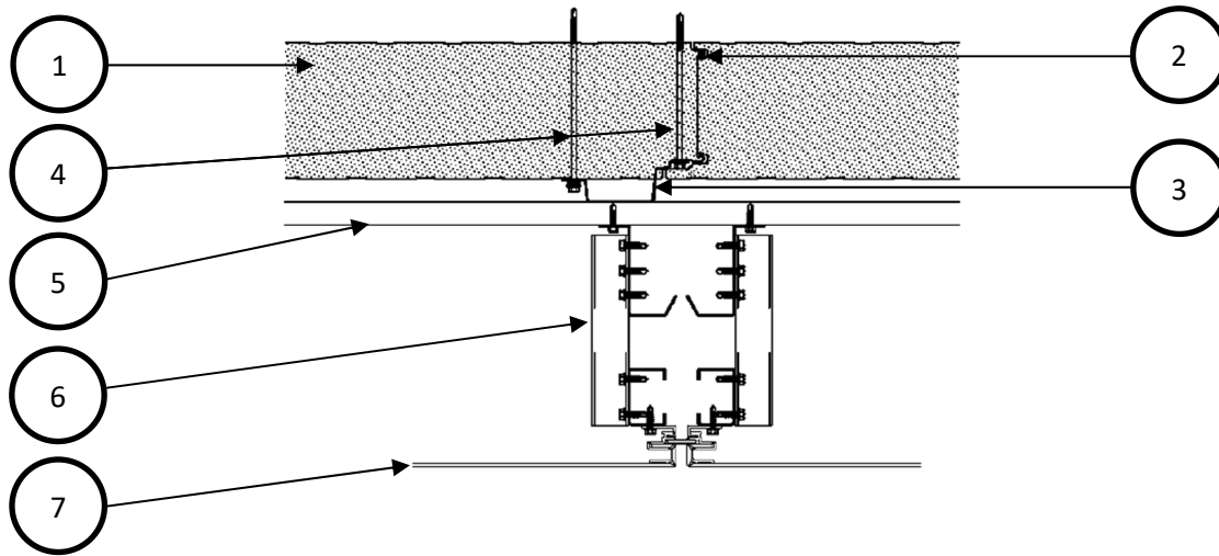
FIG 1. Vertical Joint
