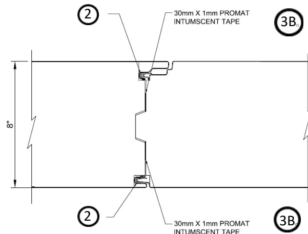
Figure 3. 8-in. Panel Intumescent Installation
