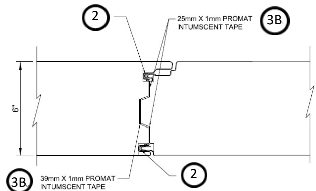
Figure 2. 6-in. Panel Intumescent Installation
