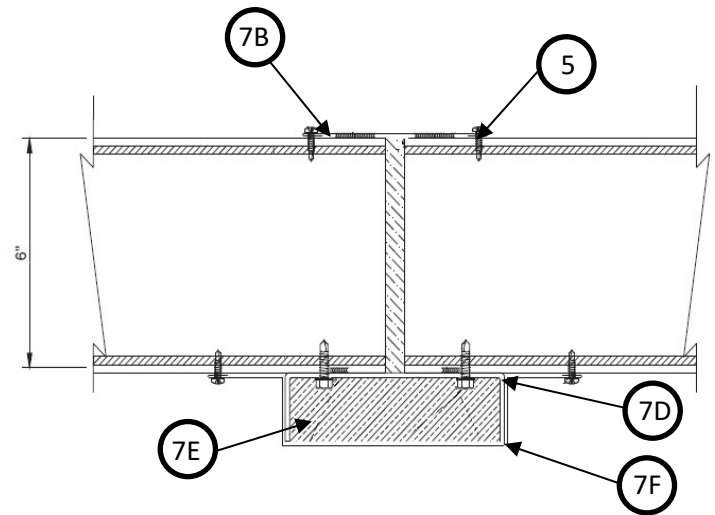
Figure 4: Butt Joint W/No Hanger
