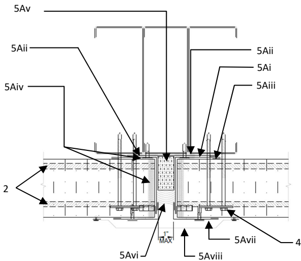
Figure 3. Butt Joint (Horizontal)
