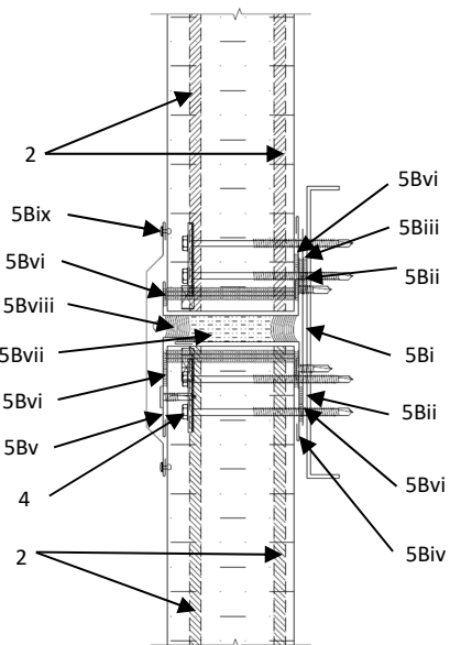
Figure 4. Stack Joint (Vertical)
