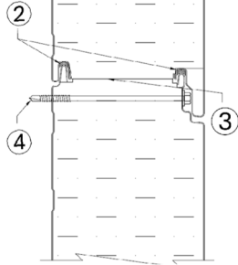
Figure 1. Standard Panel Joint (Horizontal)
