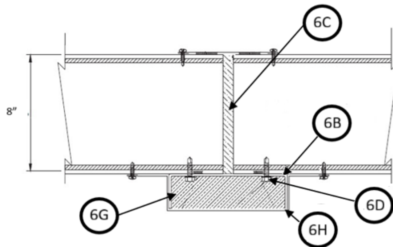
Figure 4. Butt Joint W/No Hanger
