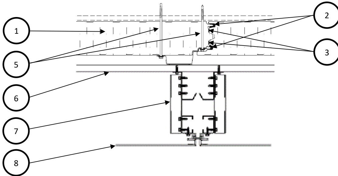
FIG 1. Vertical Joint
