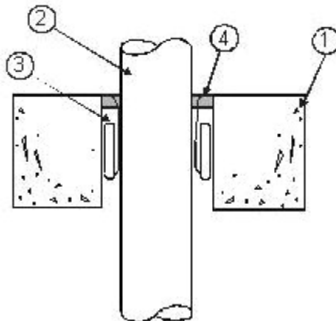
Figure 1. Penetration Detail
