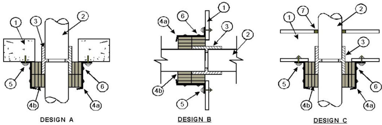
Figure 1. Penetration Detail
